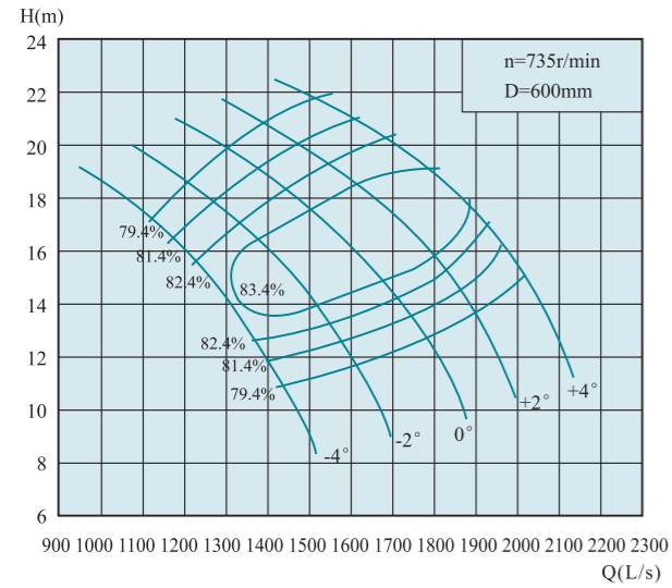
800QH-40
