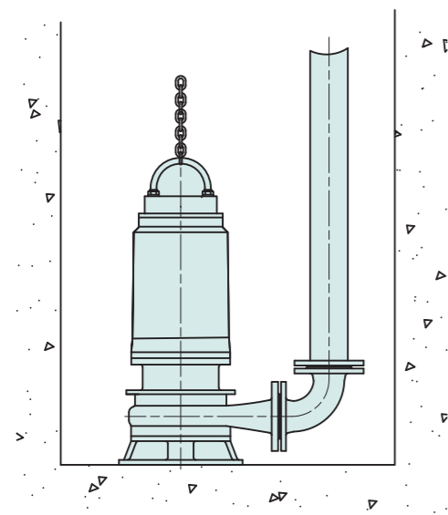
移动式硬管安装 Movable Hard Pipe Installation
