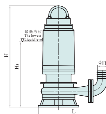
软管联接尺寸 Soft pipe connection dimension
