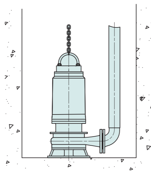
移动式软管安装 Movable Soft Pipe Installation
