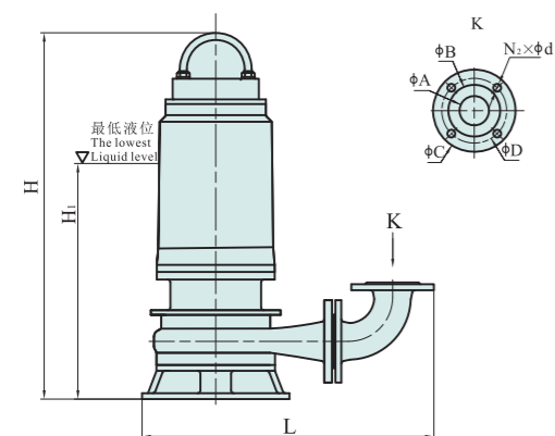
硬管联接尺寸 Hard pipe connection dimension
